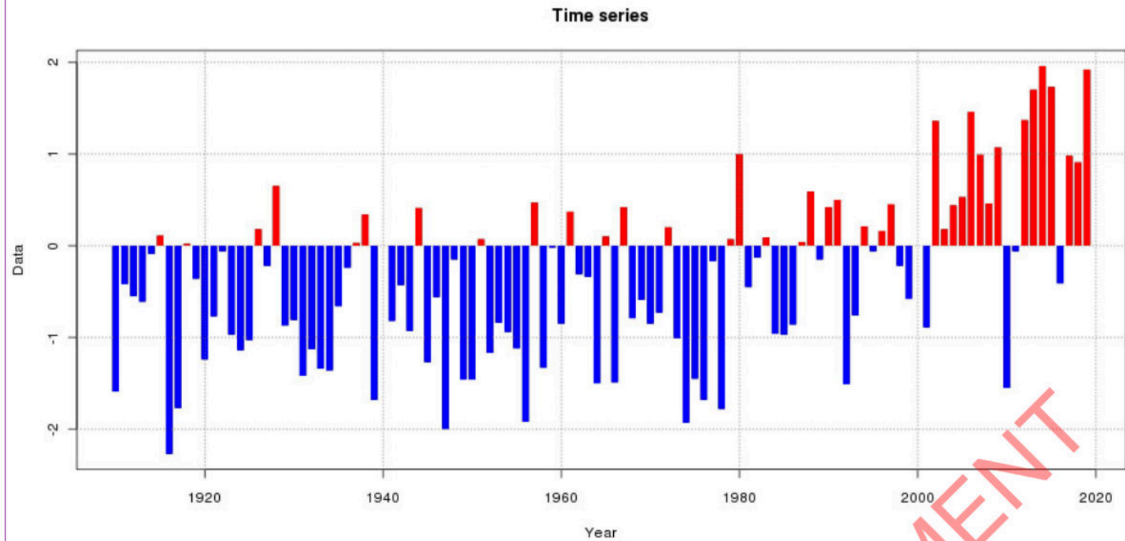
Figure 12: Graph of the spring mean maximum temperature anomaly (difference from the 1961–1990 average) for Australia from 1910 to 2019.
